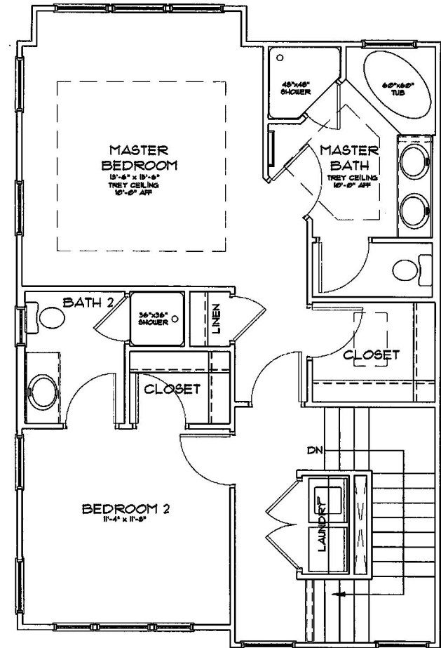
2nd Level
