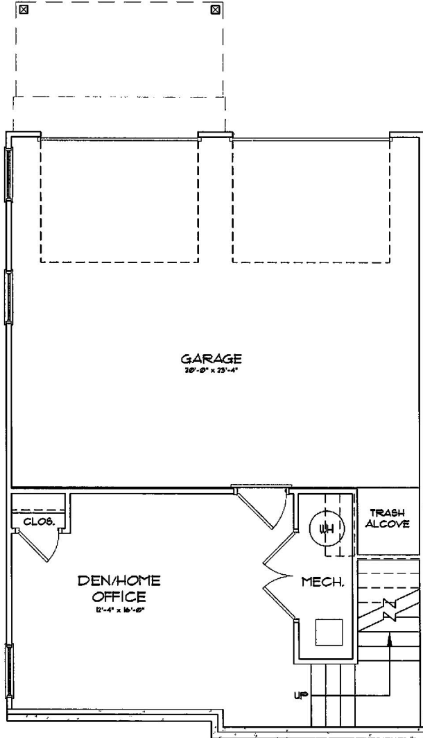
Basement Level
