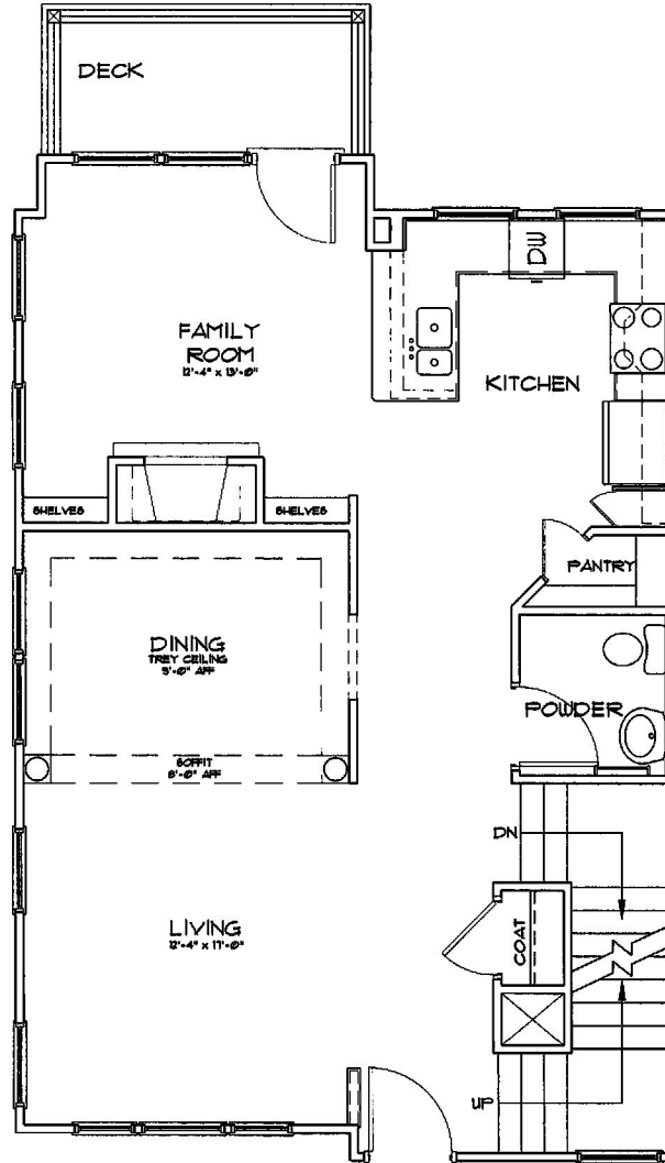
Floor Plan Typical of Units:
