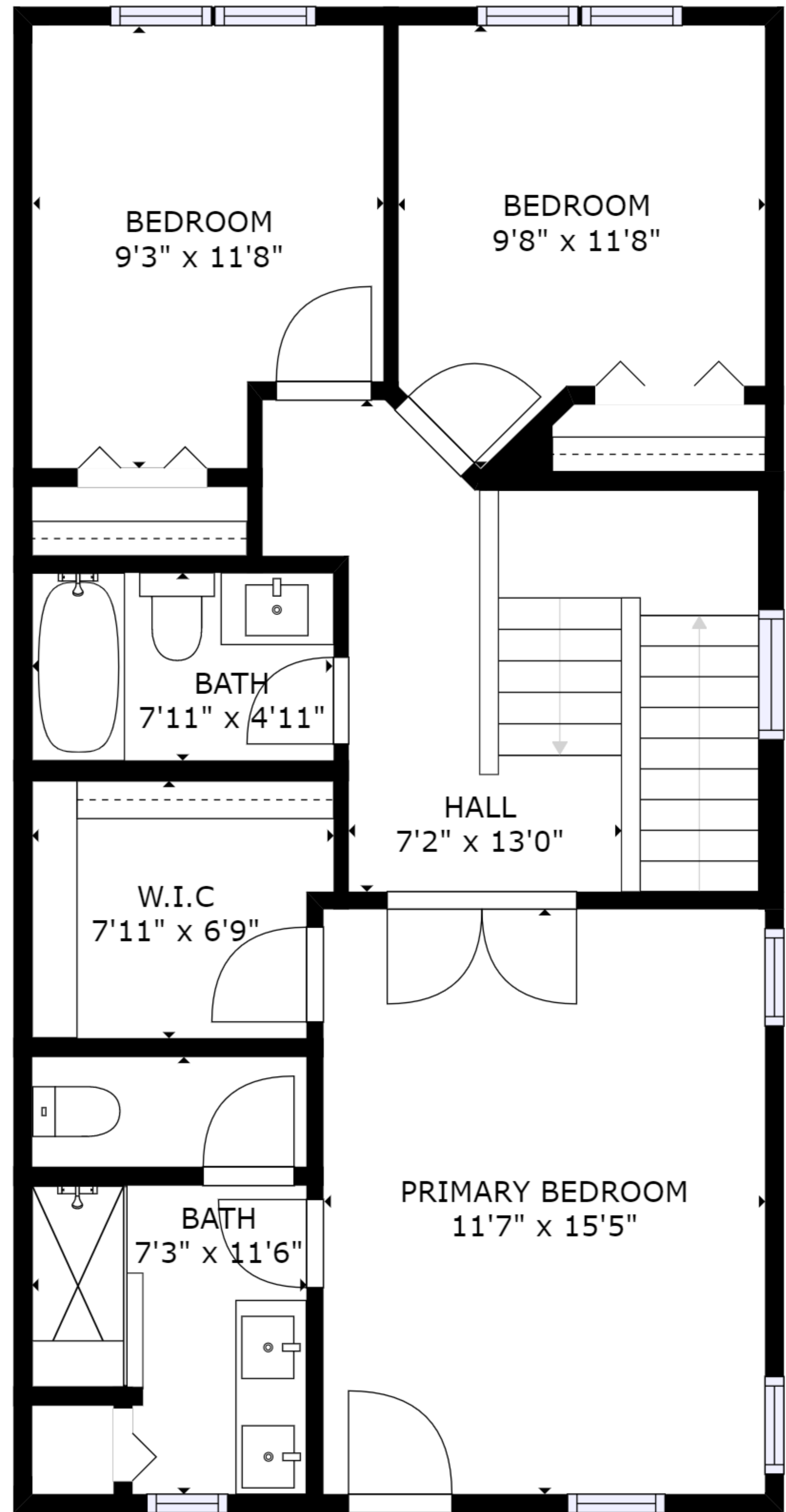
FLOOR 2
